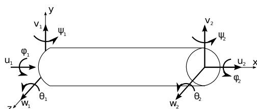
Fig. 3. 3D Timoshenko beam displacements.
