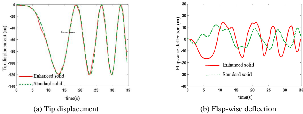
Fig. 13 Comparison between Enhanced and standard solid elements
