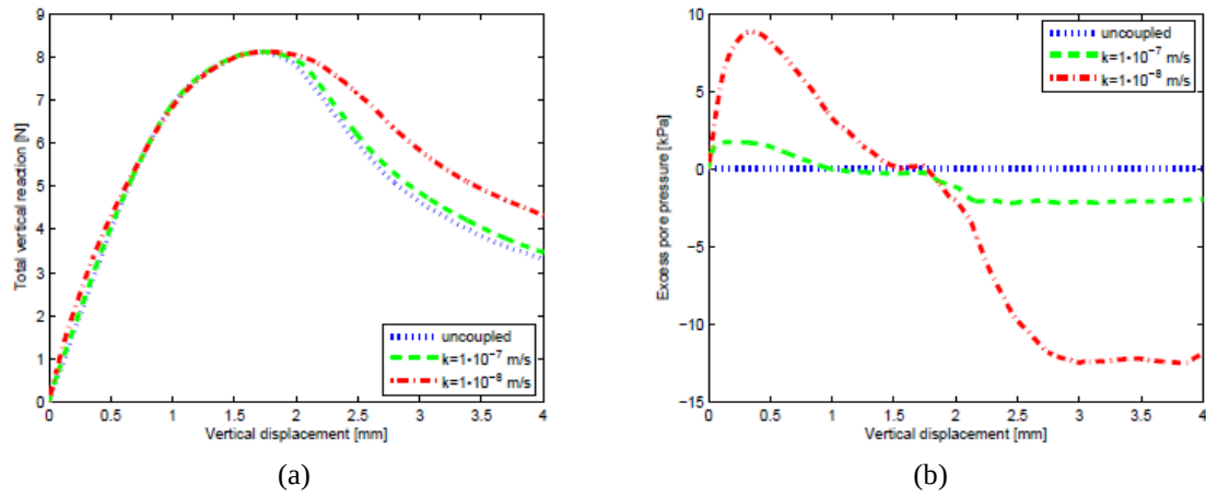
Fig. 9 Compression test (a) total vertical reaction (b) excess pore pressures ( v=1\cdot 10^{-6} m/s)
