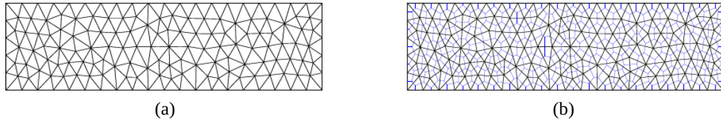
Fig. 11 Discretization of the specimen (a) mesh (b) Voronoi diagram
