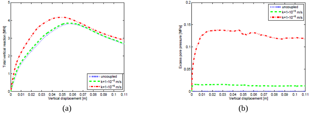
Fig. 15 Coupled soil-foundation systems (a) total vertical reaction (b) excess pore pressures ( v = 5 \cdot 10^{-5} m/s)
