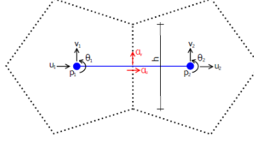
Fig. 1 Timoshenko beam finite element with enhanced kinematics
