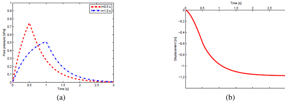
Fig. 4 Discrete lattice model (a) excess pore pressures (b) vertical displacement of the top of the sample
