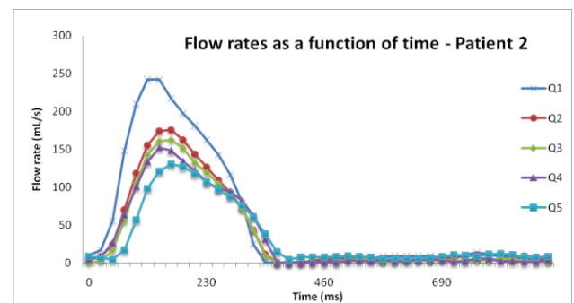
Figure1: Flow rates recordings at different locations along the aorta, after surgery, for one of the patient of the study
