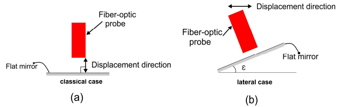
Fig. 2. Schematic diagrams for the displacement directions.
