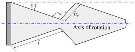
Fig. 8. Geometric form of two steps in the cones assembled grating.
