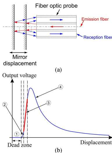
Fig. 1. Measurement principle of the fiber-optic displacement sensor.
