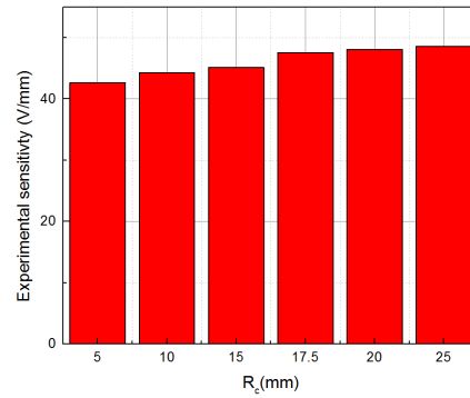
Fig. 7. Experimental sensitivity for several radii of curvature.
