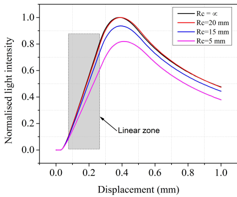
Fig. 4. Response curves for several radii of curvature.
