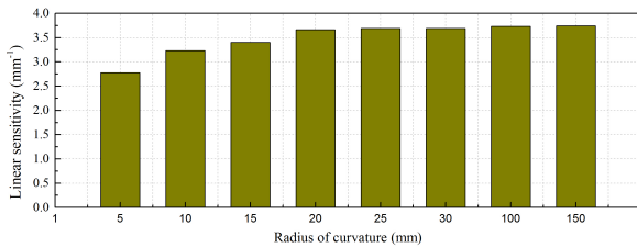
Fig. 5. Linear sensitivity for several radii of curvature (geometric model results).
