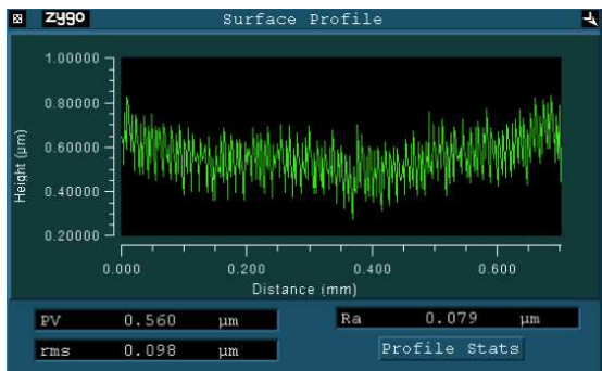
Fig. 13. Surface roughness for the first step using the interferometric microscope New View 200.
