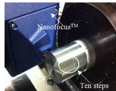
Fig. 11. Geometric characteristics with the Nanofocus TM .
