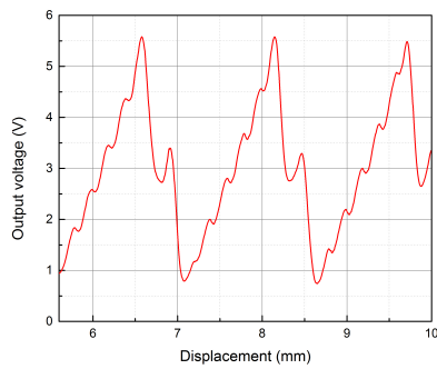
Fig. 16. Output voltage as a function of the grating in translation of 0.1 mm/s and in rotation at 0.5 rps.
