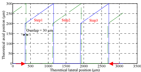
Fig. 9. Geometric model result for the cones grating sizing.
