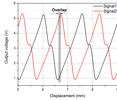
Fig. 14. Output voltage as a function of the grating displacement at 0.5 \text{ mm/s}
