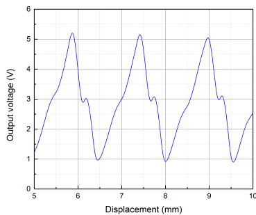
Fig. 17. Output voltage as a function of the grating in translation at 0.5 mm/s and in rotation at 1 rps.
