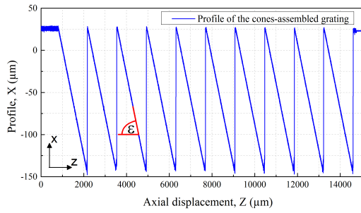
Fig. 12. Geometric profile of the cones assembled grating after fabrication.
