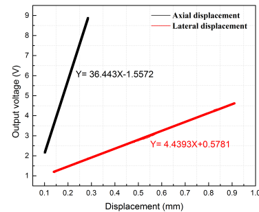
Fig. 15. Axial displacement and lateral displacement in front of one step in the cones assembled grating.
