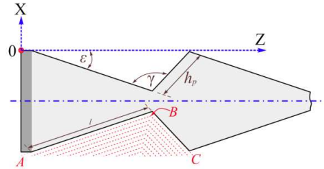
Fig. 10. Schematic diagram for the machining technique.
