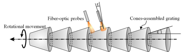
Fig. 3. Schematic diagram of the cones assembled grating associated to the fiber-optic probes.
