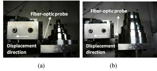
Fig. 6. Experimental setup: (a): piece (A), (b): piece (B).
