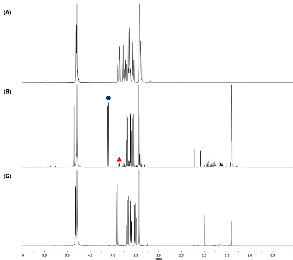
Figure 2. ^1\text{H-NMR} spectra of (A) methyl \alpha -glucoside (starting material); (B) crude mixture without \text{NaHCO}_3 after 17 days, (C) crude mixture with 1 eq. \text{NaHCO}_3 after 24 h. Comparison between H-5 signal of \alpha -methylglucuronic acid (●) and H-6 of methyl \alpha -glucoside (▲) allows the evaluation of the conversion. From (B) to (C), the H-5 signal shifted from 4.1 to 3.9 ppm because of the basic pH (sodium carboxylate instead of carboxylic acid).
