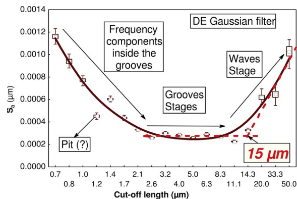
Fig. 1. Mean values and associated confidence intervals of the arithmetic mean deviation S_a as a function of the cut-off length, using a Robust Gaussian band-pass filter (DE), for the superfinished specimens.
