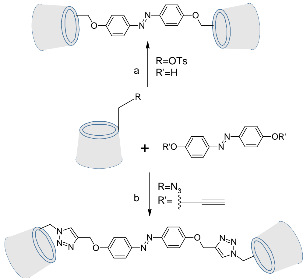
Figure 18. Ways of syntheses. a. \text{Cs}_2\text{CO}_3 , DMF, 90^\circ\text{C} , 24 h; b. (\text{EtO})_3\text{P}\cdot\text{CuI} , DMF, 100^\circ\text{C} , 2 h.
