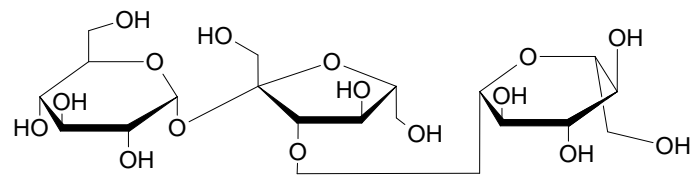
Figure 4. Melecitose structure.
