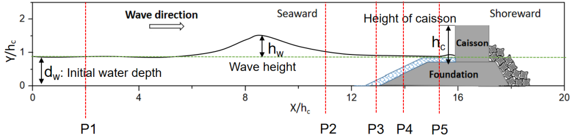
Figure 5: Schematic illustration of the computational domain. Wave type: solitary wave; wave height h_w=6\text{ m} ; water depth d_w = 10\text{ m} ; armour layer thickness T_a=2\text{ m} ; breakwater caisson height h_c=13\text{ m} ; caisson position: x/h_c=15.96 . The precise location of gauges P1-P5 is 2h_c , 11h_c , 13h_c , 14h_c and 15.5h_c (m), respectively.
