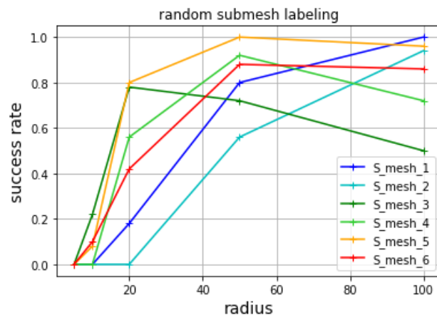
Figure 9: S_{mesh_i} local regions labeling with OLS model fitting method.
