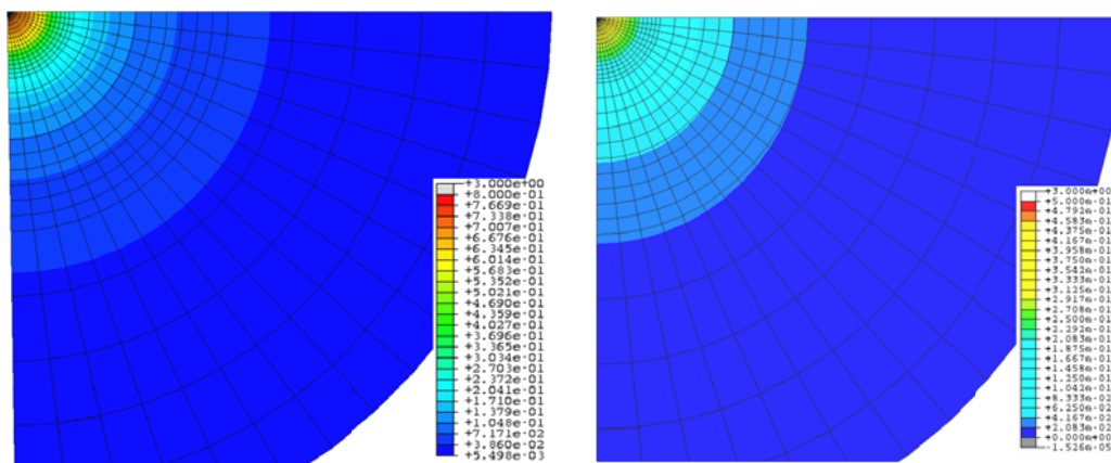
Figure 12: Isolines of numerical \Delta z for the PMMA (left) and the bone along the longitudinal axis (right)
