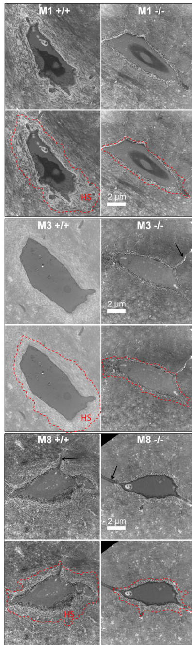
Fig. 1. TEM micrograph ( \times 11,000 ) of osteocytes located in the endosteal portion of the femur from one-month (M1), three-month (M3) and 8-month (M8) old WT (+/+) and TIEG1 KO (-/-) mice. The hypomineralized surface (HS) is located between the border of the cell and the dotted line. Black arrow indicates canaliculi. Bar = 2 \mu\text{m} .
